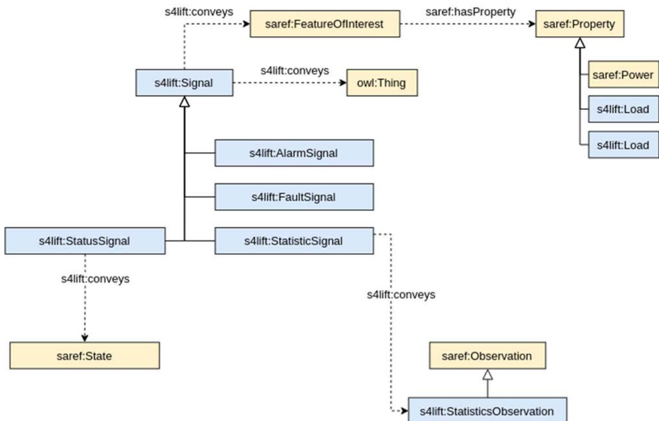
Figure 6.2.5-1: Signal model
