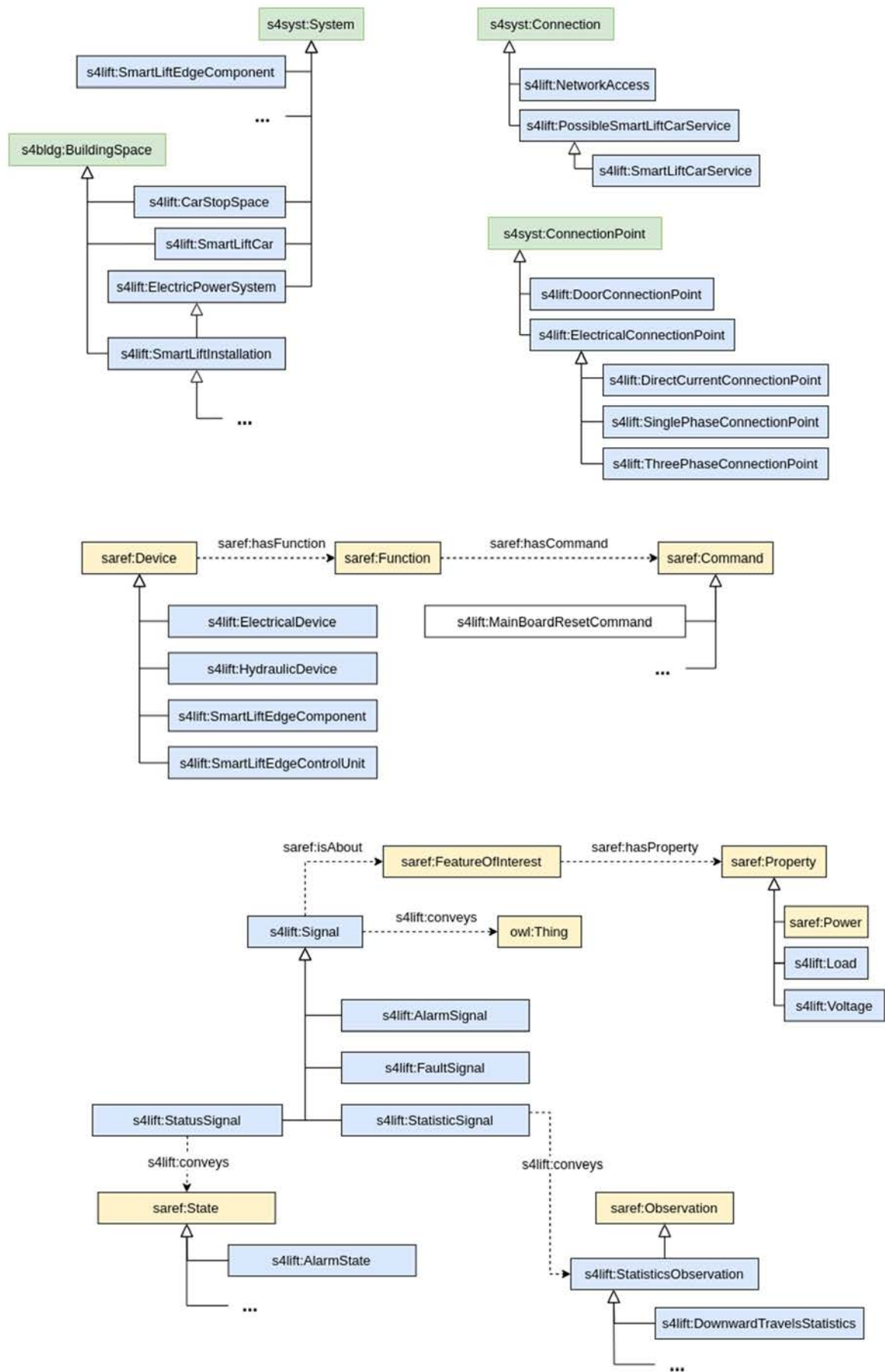
Figure 6.2.1-1: SAREF4LIFT overview
