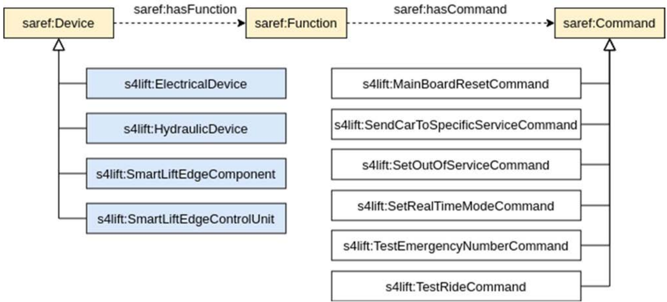
Figure 6.2.3-1: Command model
