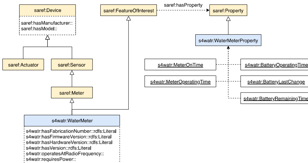
Figure 4: Water meter model
