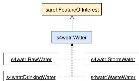
Figure 8: Water types model
