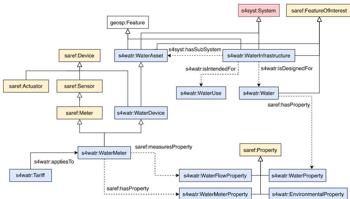
Figure 2: SAREF4WATR overview, Water-related terms
