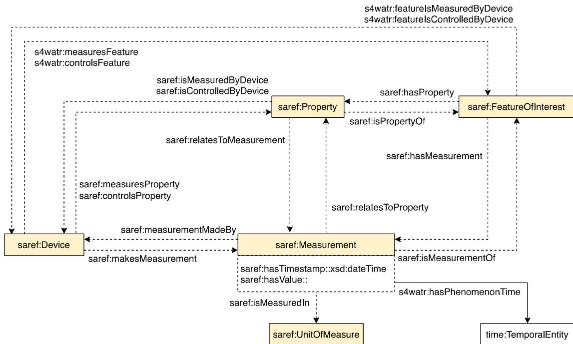
Figure 3: Measurement model
