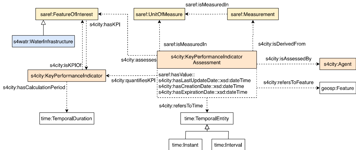
Figure 12: Key Performance Indicator model
