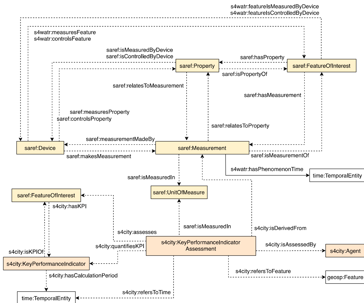
Figure 1: SAREF4WATR overview, Measurements and KPIs
