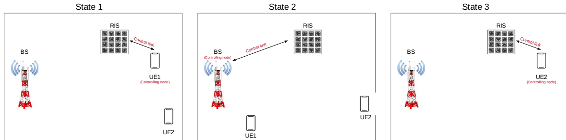
Figure 6.3.0-1: Illustration of updating the RIS management
