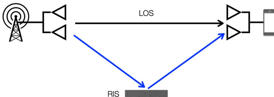
Figure 5.2-1: Utilizing RIS with MIMO: multiplexing and interference management
